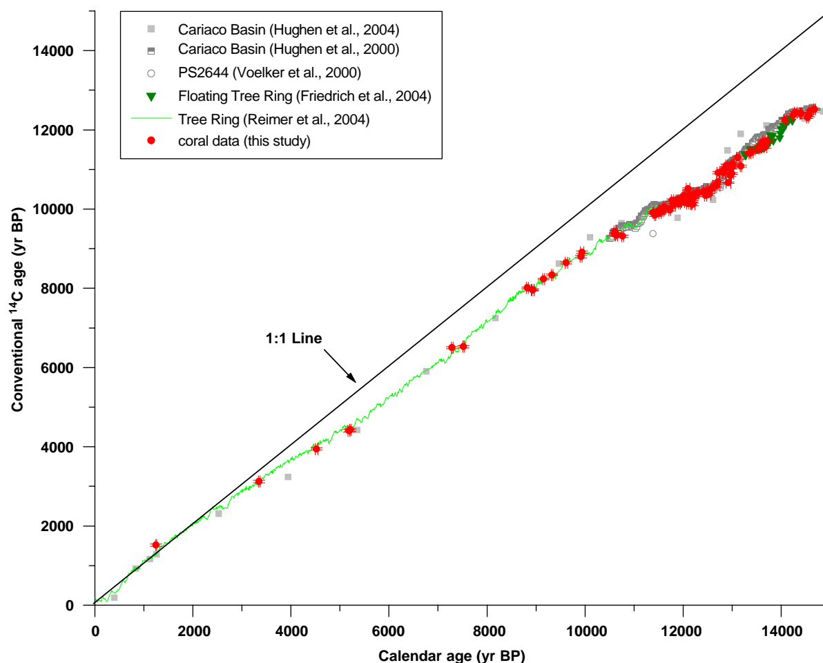
Fig. 2. Comparison of our coral data to the tree ring records of Reimer et al. (2004) and Friedrich et al. (2004) and the marine sediment data with calendar chronologies based on overlap with the tree ring data set and correlation to the oxygen isotope record in Greenland ice cores (Hughen et al., 2000, 2004a; Voelker et al., 2000). Note the consistency of our coral data with Friedrich et al.'s (2004) floating tree ring chronology, and where both diverge from the Cariaco (Hughen et al., 2000, 2004b) varved sequence between 13,300 and 14,000 yr BP. Figure zoom feature available at: http://www.radiocarbon.ldeo.columbia.edu .
