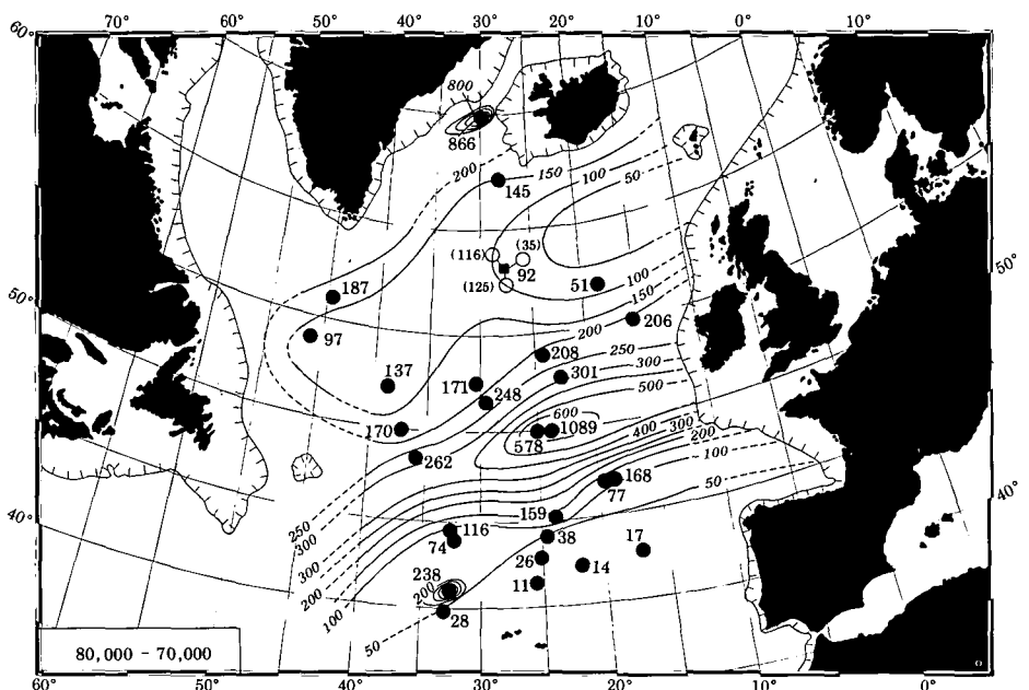
Figure 4C. Mean deposition rate from 80,000 to 70,000 B.P. (isotopic substage 4). This pattern (with Figs. 4D through 4G) is basic glacial mode of deposition. Major shift in depositional pattern and large increase in total abundance has occurred since intervals shown in Figures 4A and 4B.
