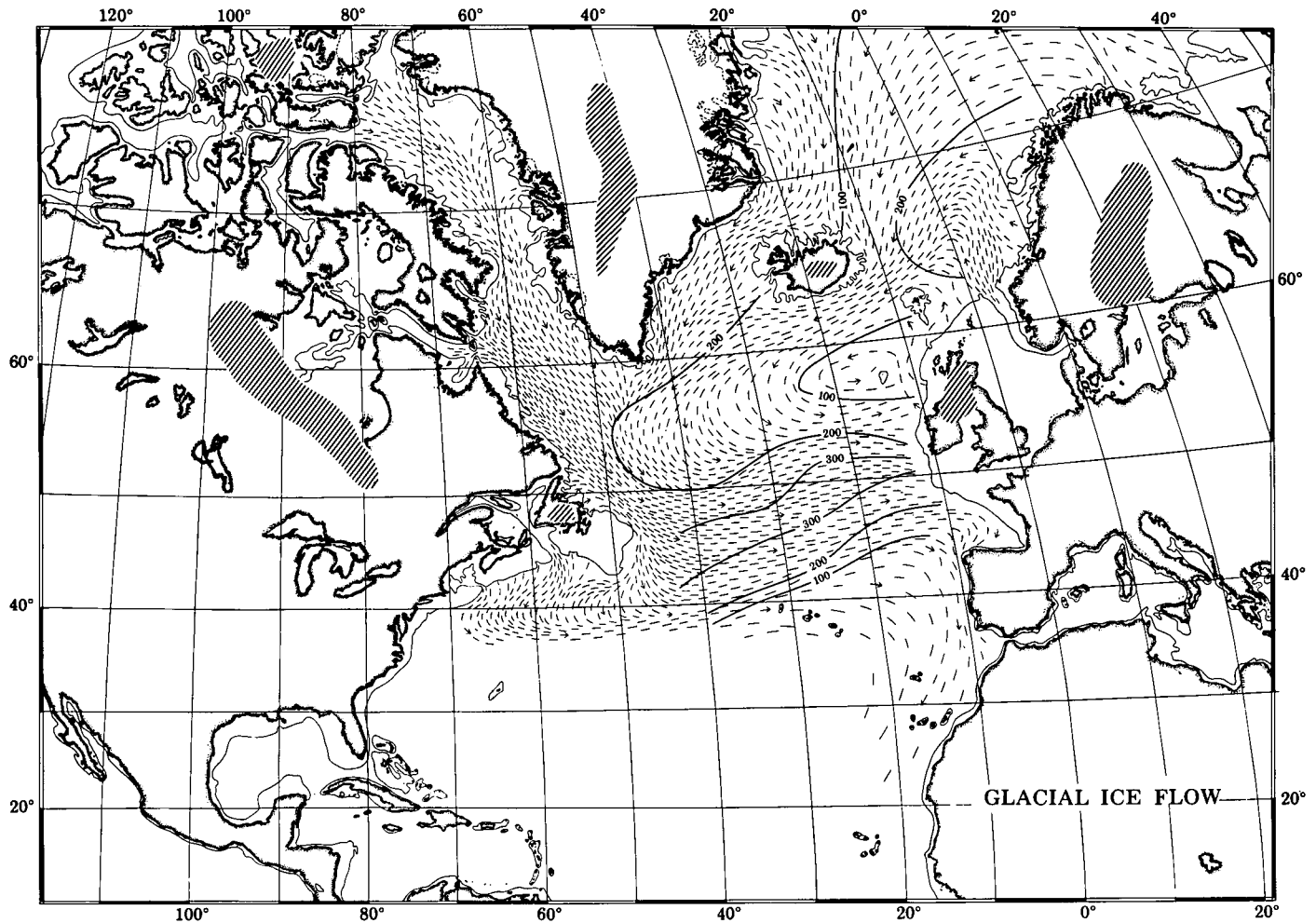
Figure 7B. Inferred mean paths of distribution of ice-rafted detritus during a main glacial regime. Diagonal-ruled areas = spreading centers of continental ice sheets. Oceanic distribution pattern (dashed lines) is basically cyclonic as during interglacial regime and at present.
