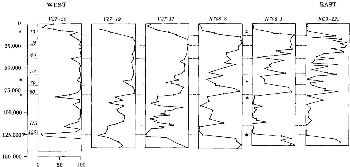
Figure 6. West-east transect across subpolar North Atlantic at lat 50^{\circ} to 55^{\circ} N. Plot shows abundance of Globigerina pachyderma (s.) as percentage of total planktonic foraminiferal population. Cores plotted to time between same control levels (marked by asterisk) used to plot noncarbonate sand (Fig. 3). Ice-rafting intervals mapped in Figures 4A through 4G marked by dashes. Faunal evidence shows that waters to east near Great Britain stayed warmer than those to west in Labrador Sea near Greenland during all climates.
