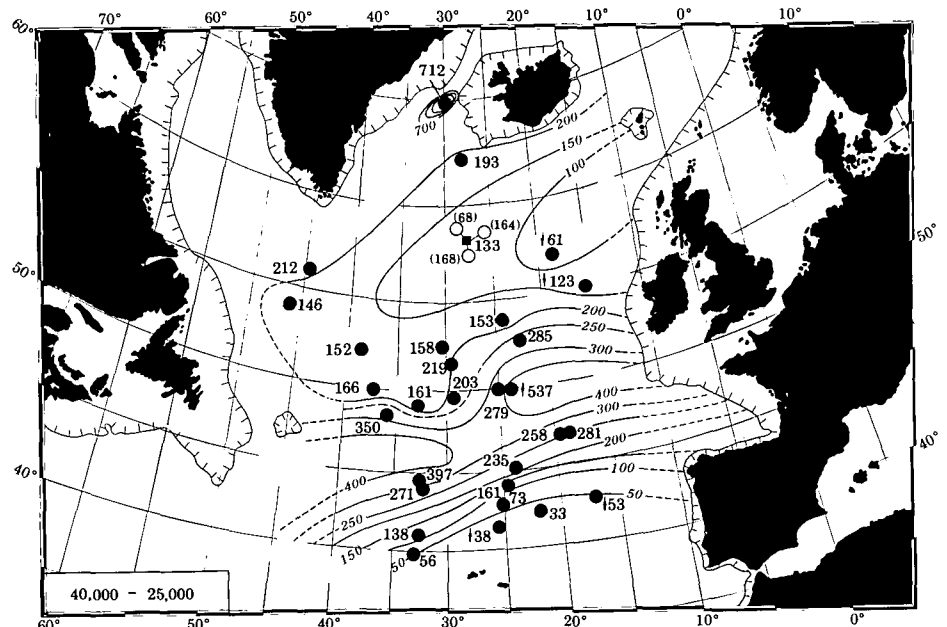
Figure 4F. Mean rate of deposition from 40,000 to 25,000 B.P. (upper part of isotopic stage 3).
