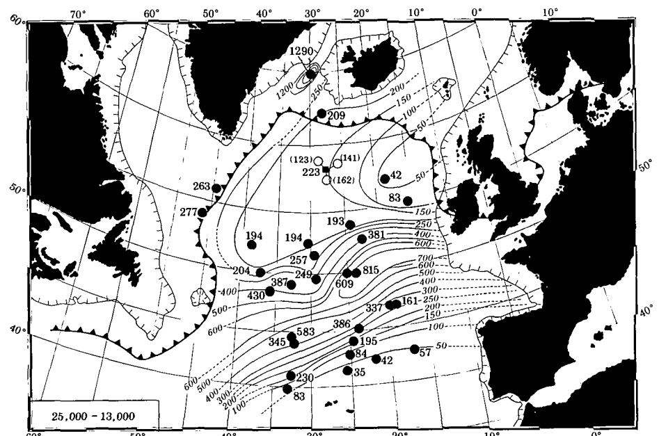
Figure 4G. Mean rate of deposition from 25,000 to 13,000 B.P. (isotopic stage 2). Line with triangles is ice-sheet limit on continents and inferred ice limit over ocean (Hughes and others, 1977).
