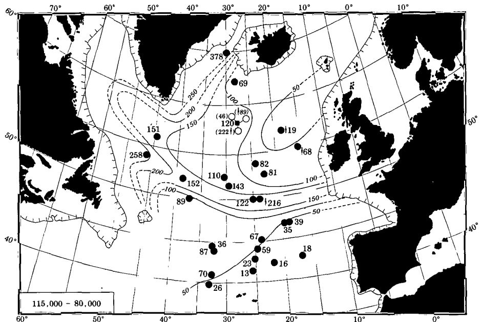
Figure 4B. Mean deposition rate from 115,000 to 80,000 B.P. (isotopic substages 5d to 5a). Slightly increased deposition evident from comparison with Figure 4A.
