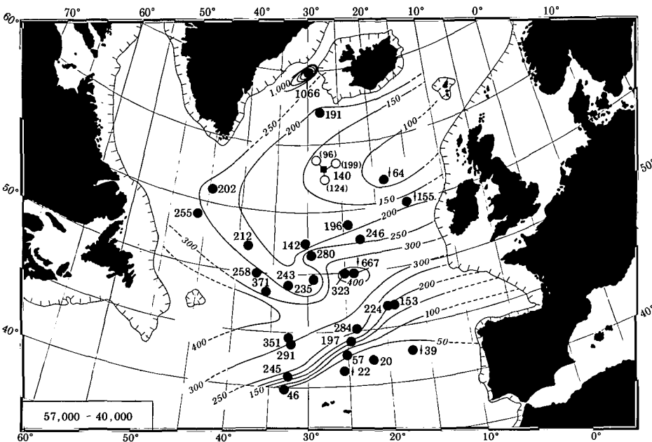
Figure 4E. Mean rate of deposition from 57,000 to 40,000 B.P. (middle of isotopic stage 3).
