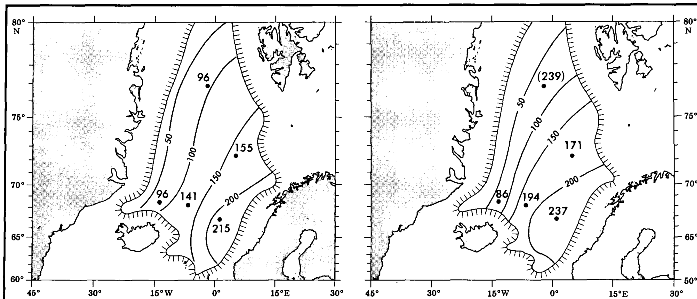
Figure 5. Left: Mean interglacial and early-glacial rate of input of ice-rafted sand, in milligrams per square centimetre per 1,000 yr from 127,000 to 75,000 B.P. in Norwegian Sea. Calculations based on data in Kellogg (1975). Hachured line delineates shelf break or slightly deeper areas thought to have been situated beneath grounded ice sheets during glacial conditions. Right: Mean main-glacial input rate from 75,000 to 10,000 B.P. in Norwegian Sea. Pattern is very similar to interglacial and early-glacial deposition (left).
