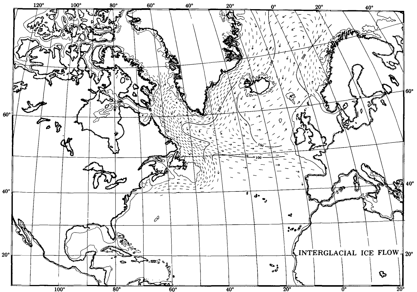
Figure 7A. Inferred mean paths of delivery of ice-rafted detritus during an interglacial regime. Sizes of continental ice masses are variable and not shown. Main distribution pattern (dashes) largely follows present-day flow of sea ice and icebergs, except for secondary flow axis to east-southeast across lat 51°N. Mean depositional rates of ice-rafted sand (in milligrams per square centimetre per 1,000 yr) cover last interglacial and early-glacial period from 125,000 to 80,000 B.P.
