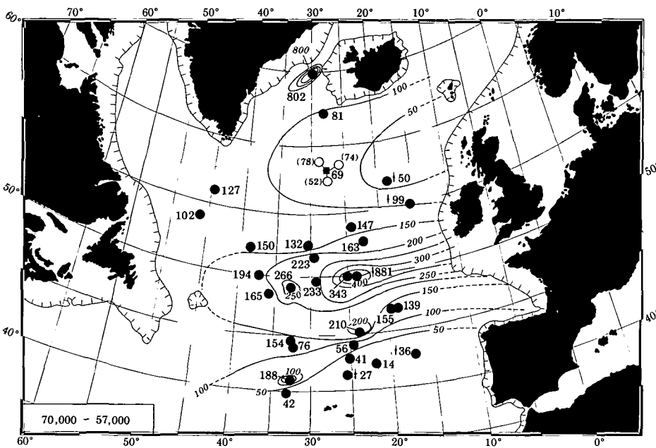
Figure 4D. Mean rate of deposition from 70,000 to 57,000 B.P. (lower part of isotopic stage 3).
