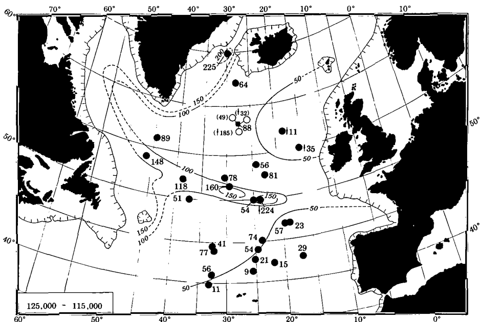
Figure 4A. Mean rate of deposition of ice-rafted sand in milligrams per square centimetre per 1,000 yr from 125,000 to 115,000 B.P. (isotopic substage 5e). Hachured line is continental shelf/slope break. This pattern (with Fig. 4B) is basic interglacial mode of deposition and largely resembles modern paths of sea ice and icebergs.
