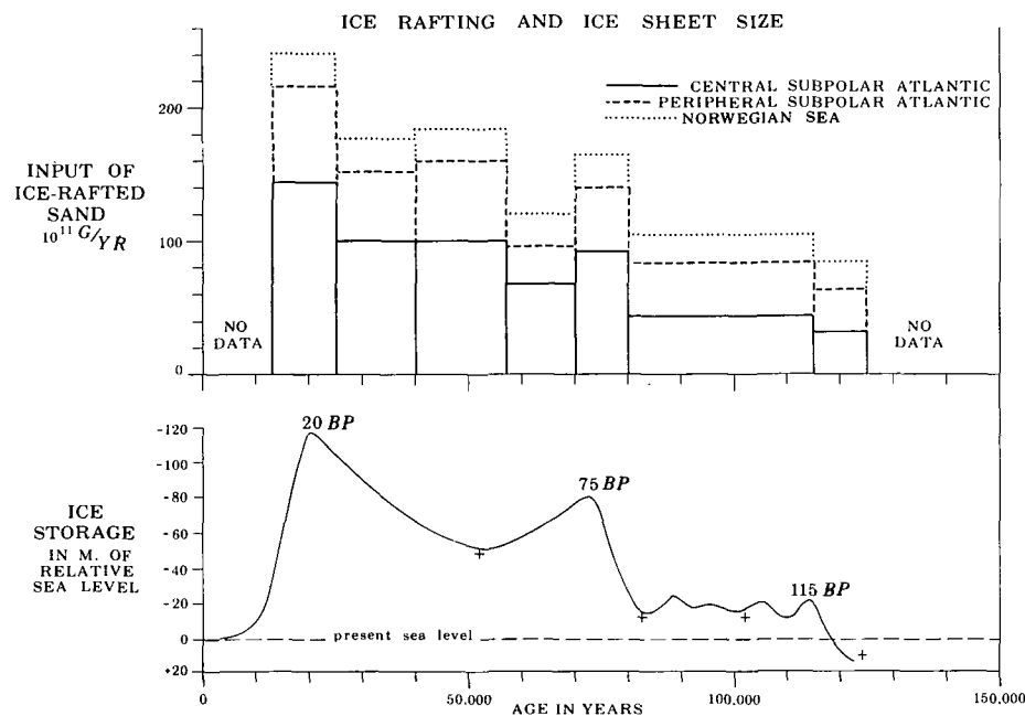
Figure 8. Total absolute input rate of ice-rafted sand during seven intervals mapped in Figure 4. Input integrated across central subpolar Atlantic outlined by heavy dashed line in Figure 1, peripheral subpolar Atlantic enclosed by dotted lines and continental slope in Figure 1, and Norwegian Sea (Fig. 5). Major increase of ice-rafting at 75,000 B.P. corresponds to southeastward shift in depositional pattern (Fig. 4). Lower curve showing isotopic evidence primarily of ice sheet growth (from Shackleton and Opdyke, 1973) matches ice-rafted changes.
