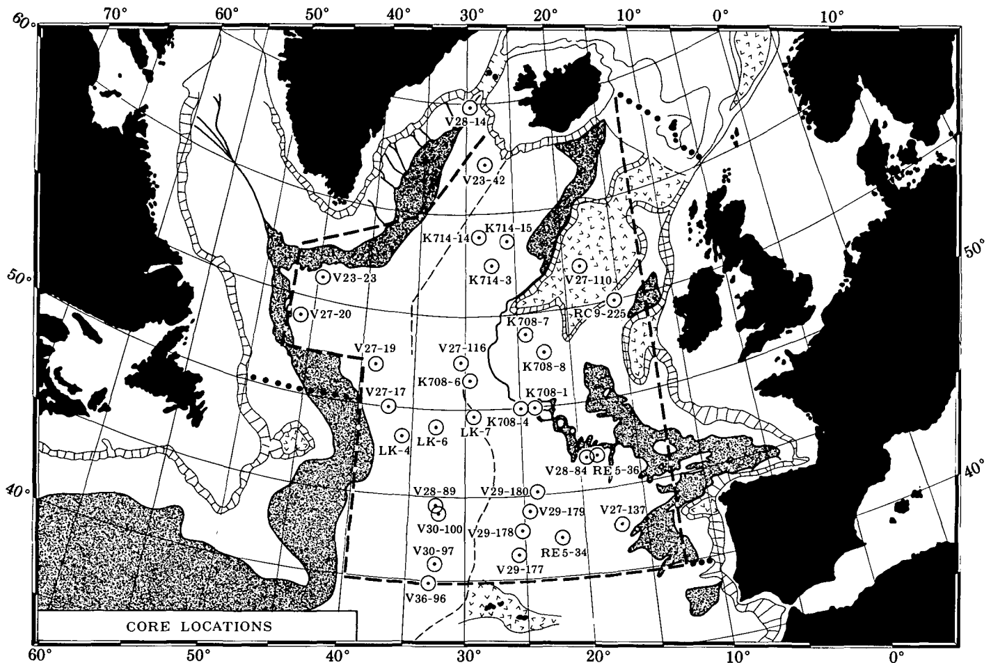
Figure 1. Locations of cores used in glacial detritus study (Table 1). Stippled pattern marks turbidite provinces: abyssal plains, fans, canyons, and channels. V pattern marks shallow offshore plateaus. Hachures delineate continental and insular slopes. Heavy dashed line encloses central subpolar area across which total ice-rafted input was integrated. Light dashed line shows mid-oceanic ridge crest. Dotted lines and continental slope (hachures) enclose additional peripheral region of ice-rafted input.
