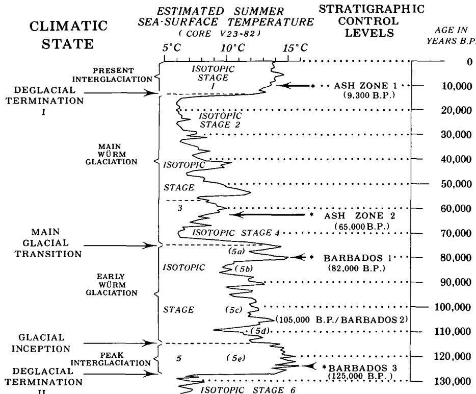
Figure 2. North Atlantic climatic curve based on estimated summer sea-surface temperatures in core V23-82 (from Sancetta and others, 1973). Levels used as control in other cores shown by asterisks and arrows on right. General Northern Hemisphere climatic conditions and prominent changes shown at left. Cores plotted to time by alignments noted in text. Placement of isotopic stages and terminations explained in text.
