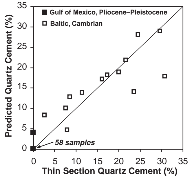
Figure 4—Comparison of predicted and measured quartz cement abundances for samples representing end members in heating rates using quartz cementation kinetics calibrated to Jurassic samples from the Norwegian continental shelf. The model provides accurate predictions for shallow Cambrian samples from the Baltic region [petrographic data from S. Bloch (1993, personal communication); burial history data from Brangulis et al. (1993)], as well as for deeply buried Pliocene–Pleistocene samples from the Gulf of Mexico Basin [petrographic data of Milliken (1985)].
