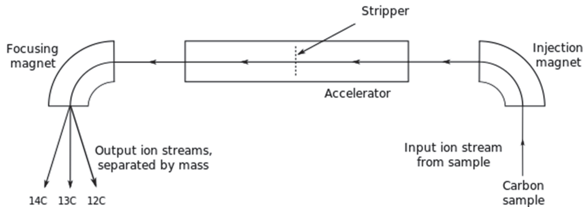
Figure 1. Simplified schematic layout of an accelerator mass spectrometer used for counting carbon isotopes for carbon dating. Aitken (1990)
