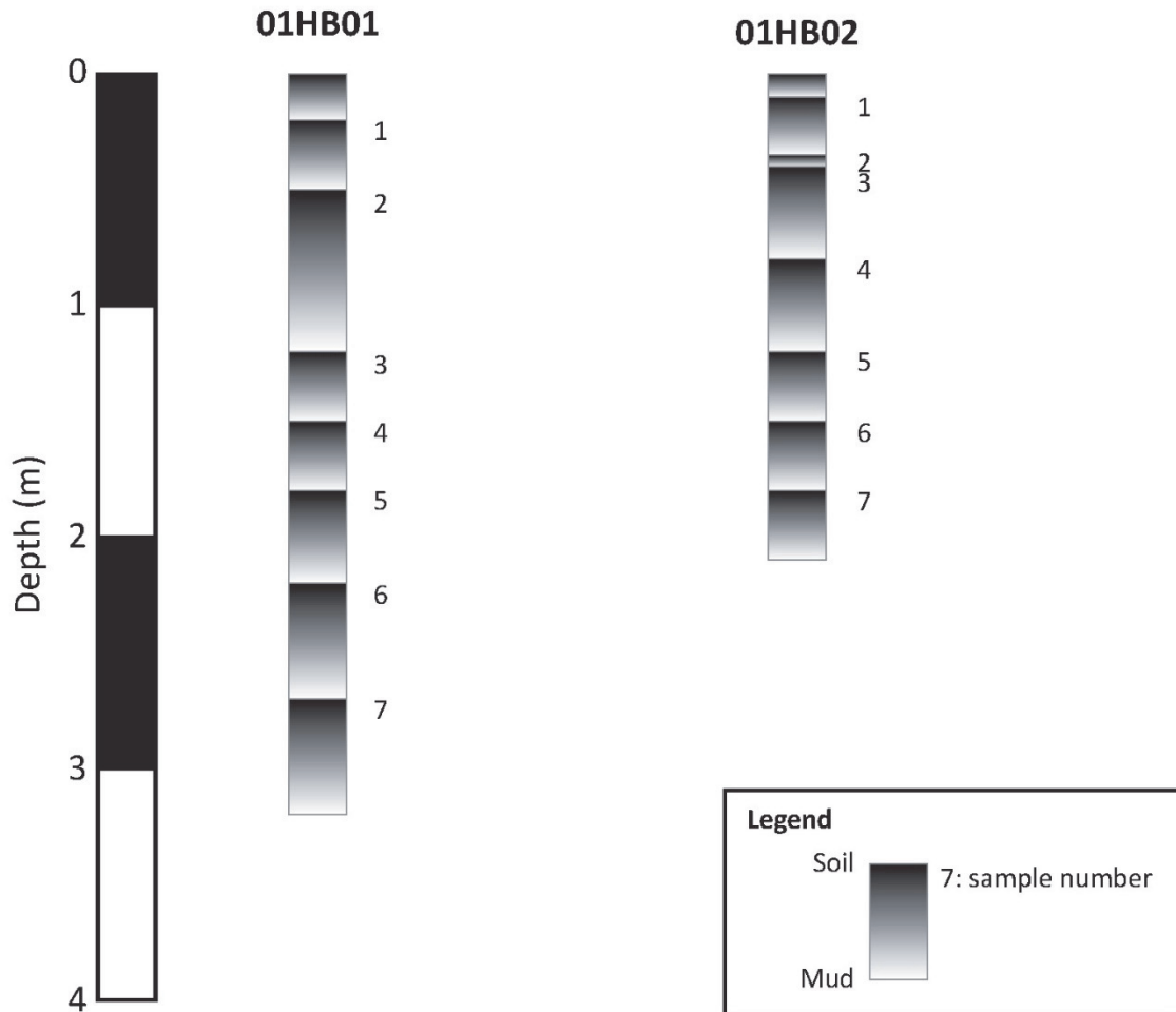
Figure 2. Sediment cores 01HB01 and 01HB02. Marsh deposits (dark gray) are overlain by muds (light gray). Sample locations are numbered, but not every sample location has a radiocarbon result.
